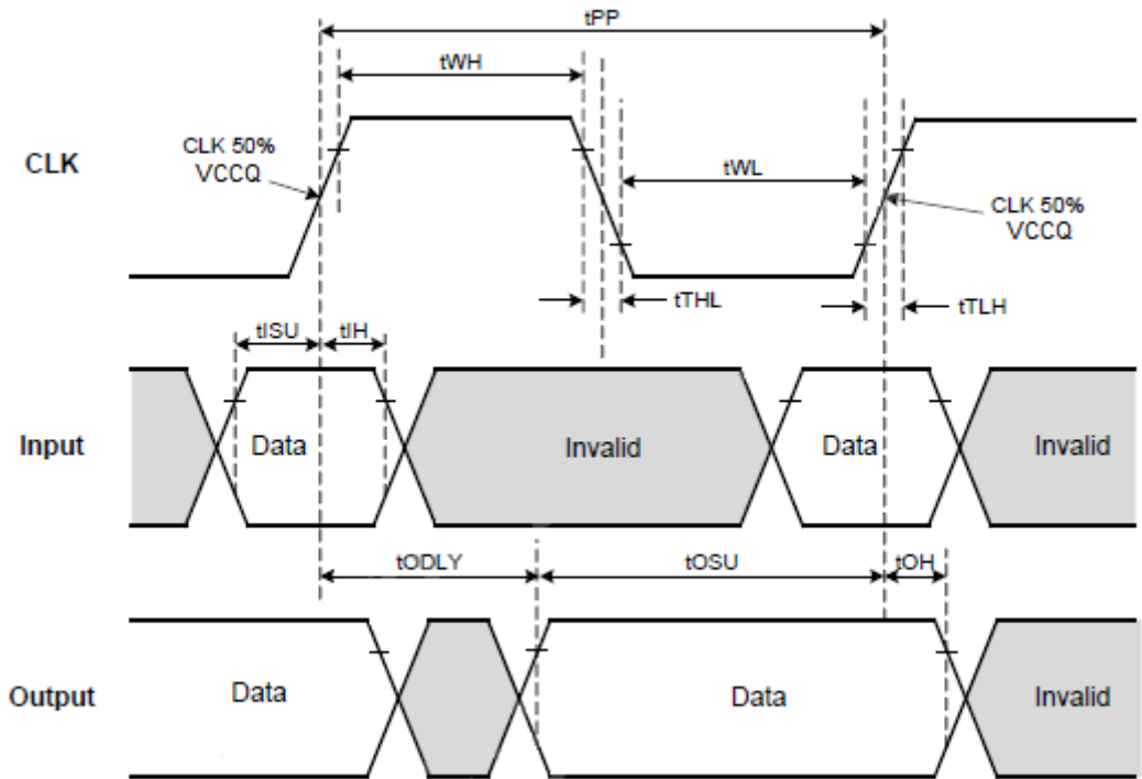
Bus Timing in Single Data Rate Mode
